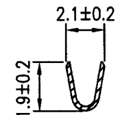
B-B SECTION
